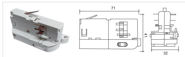
五线导轨头Five-wire rail adapter S014
