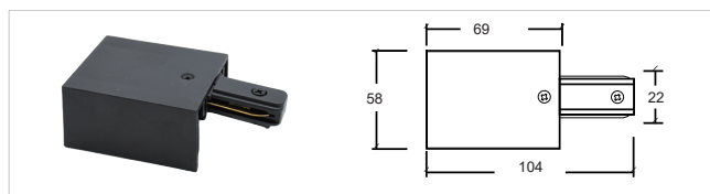
桥架尾盖 Bridge tail cover YZ6222/6317-尾盖
