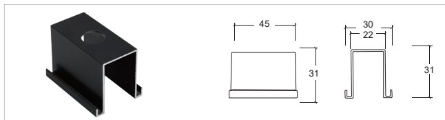
桥架吊装件C款 Track Rail Suspending Part C YZ6216/6306
