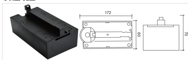
导轨盒-宽盒Rail box - wide box S033
