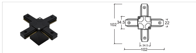
桥架吊装件B款 Track Rail Suspending Part B YZ6216/6306-B
