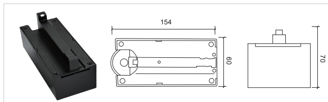
导轨盒-中盒Guide rail box - middle box S035
