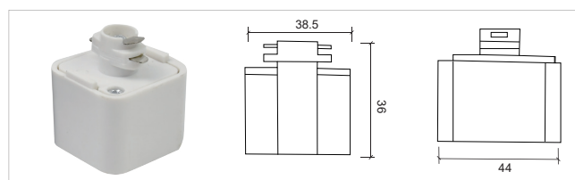
方形导轨头 Square rail adapter S015
