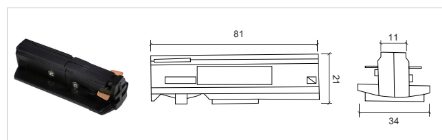
超薄导轨头 (PC) Ultra-thin rail adapter S006
