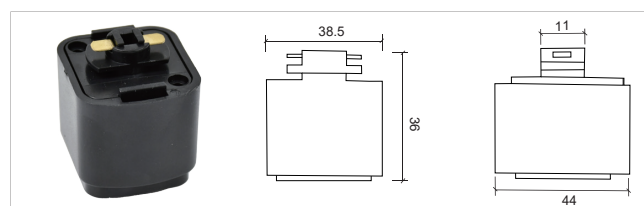
方形导轨头 Square rail adapter S015
