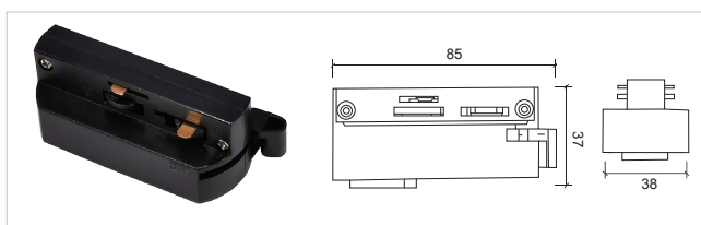
三线导轨头 Three-wire guide rail box S016
