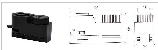
二线导轨头 Tow-line rail adapter S004-2
