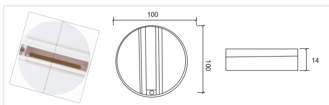
长转换盘 Conversation Base
