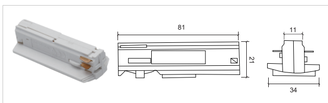
3线超薄导轨头 (PC) Ultra-thin rail adapter S007
