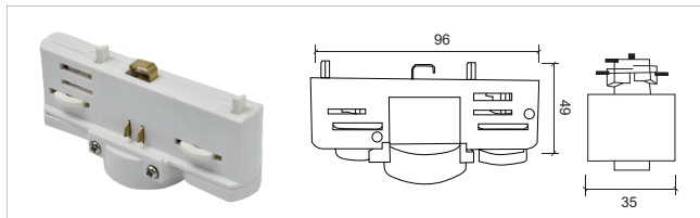
四线导轨头 Four wire guide rail S007
