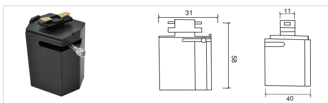
二线导轨头 Tow-line rail adapter S023
