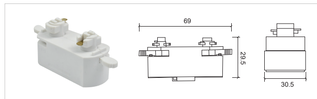
三线双柄导轨头 Three-wire double handle rail adapter S001
