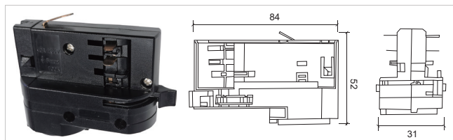
五线导轨头Five-wire rail adapter S043
