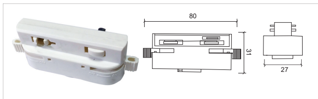
三线大双柄导轨头 Three wire large double handle rail adapter S013
