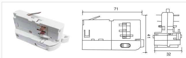
小四线导轨头 (PC) Small four-wire rail adapter S014
