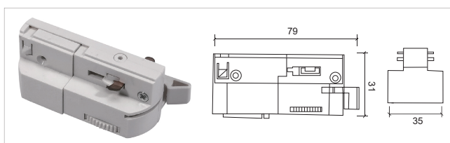
三线导轨头3 Three-wire head adapter S031
