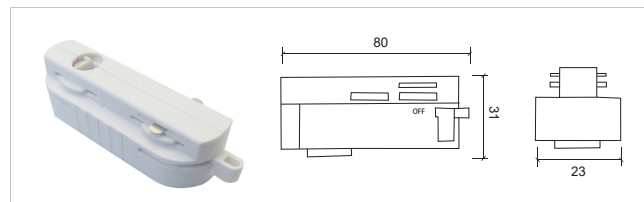
二线十字导轨 Two-wire cross rail box S005
