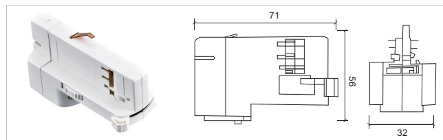
四线导轨头 短款 Four-wire conjoined (short one) S036-A
