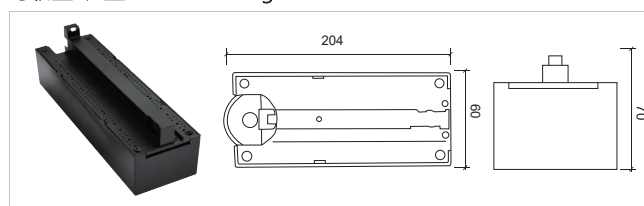
导轨盒-长盒Rail box - long box S034
