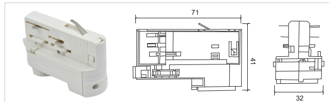
四线导轨头 (PC) Four-wire rail adapter S002
