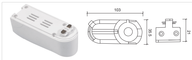
二线小导轨盒 Two-wire small rail box S004
